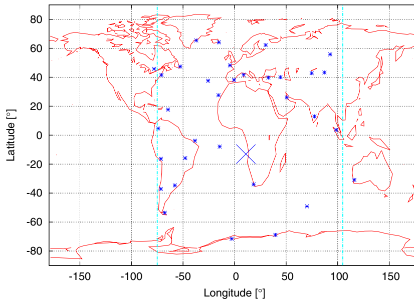
Fig. 2. Distribution of the GPS reference stations that allow the detection of the Halloween storm at about 11 UT, on 28th October, 2003. The large cross-marks the Sun's subsolar point and the two vertical lines roughly delimit the sunlit area.
